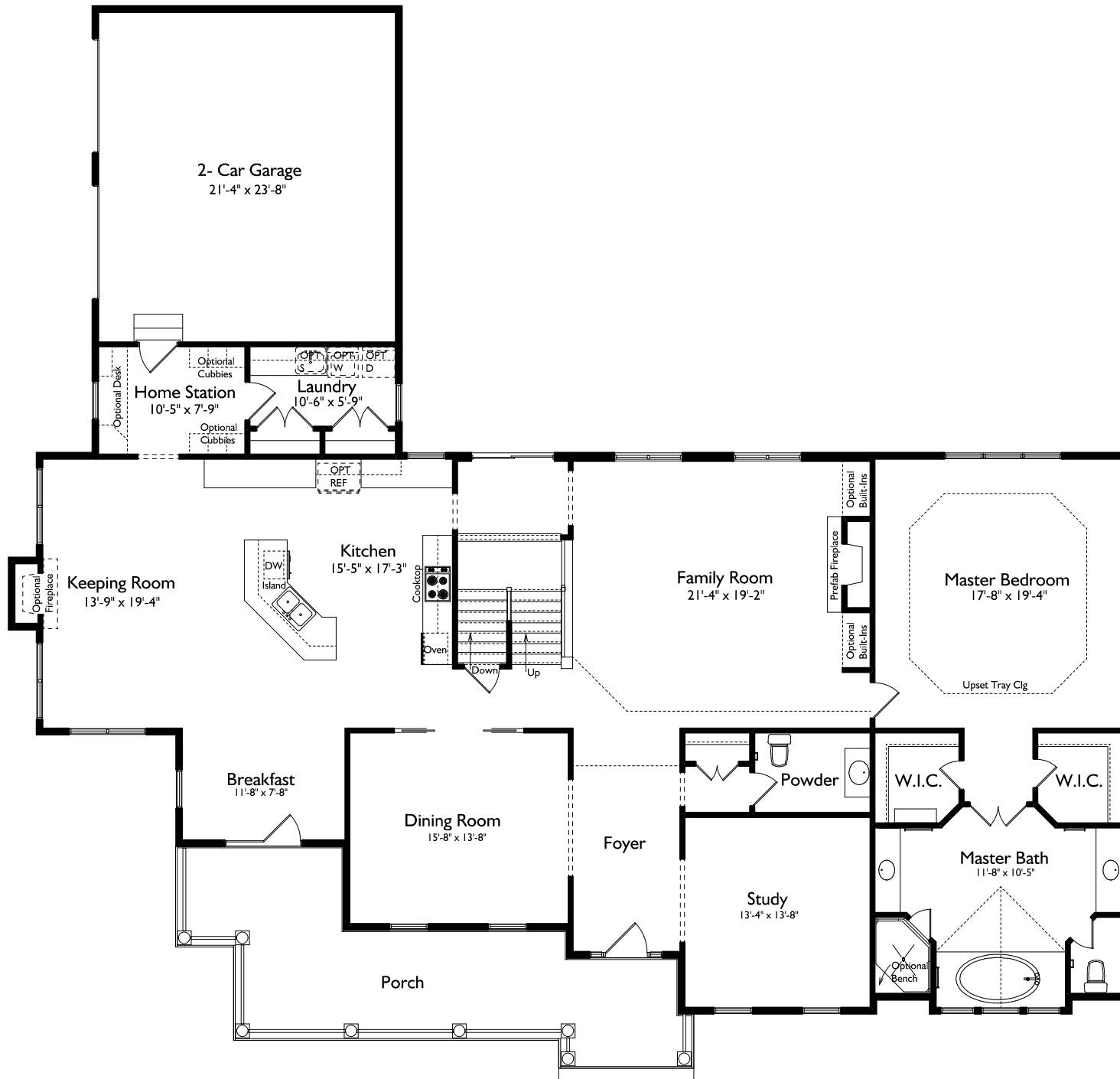
First Floor Plan 9' Wall Height Magnolia
