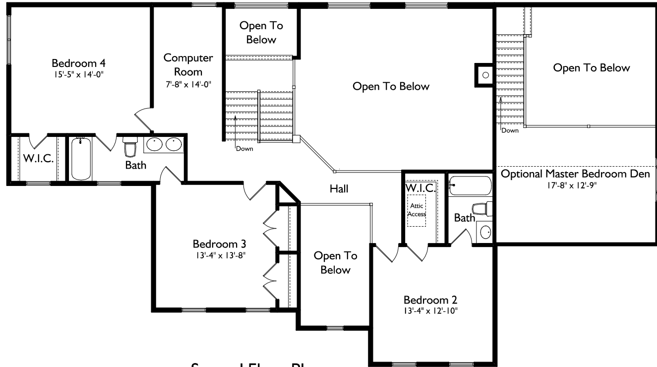
Second Floor Plan 9' Wall Height
