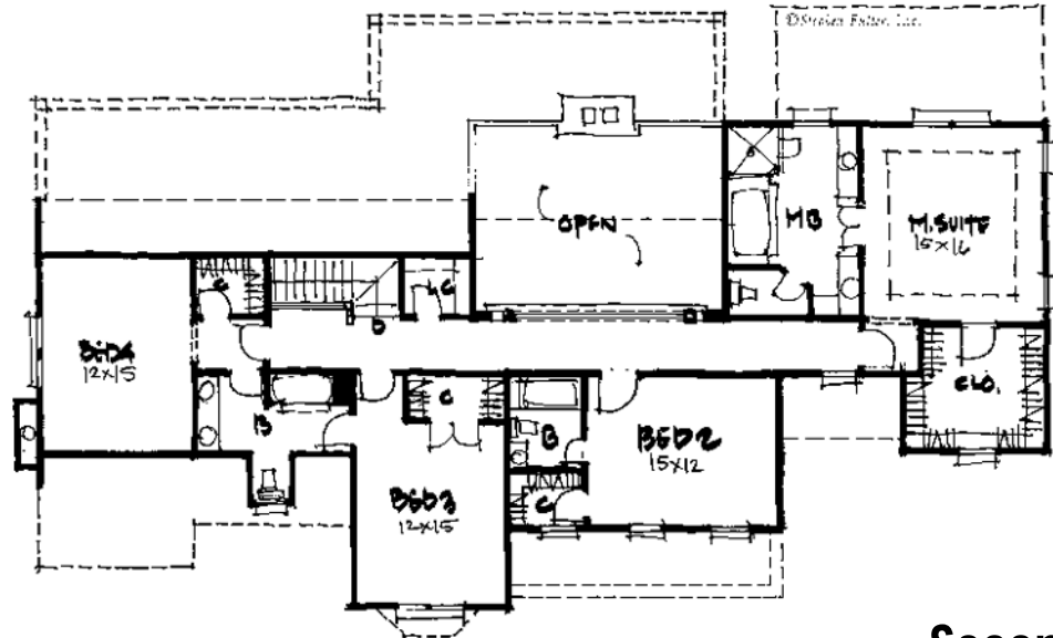
Second Floor
