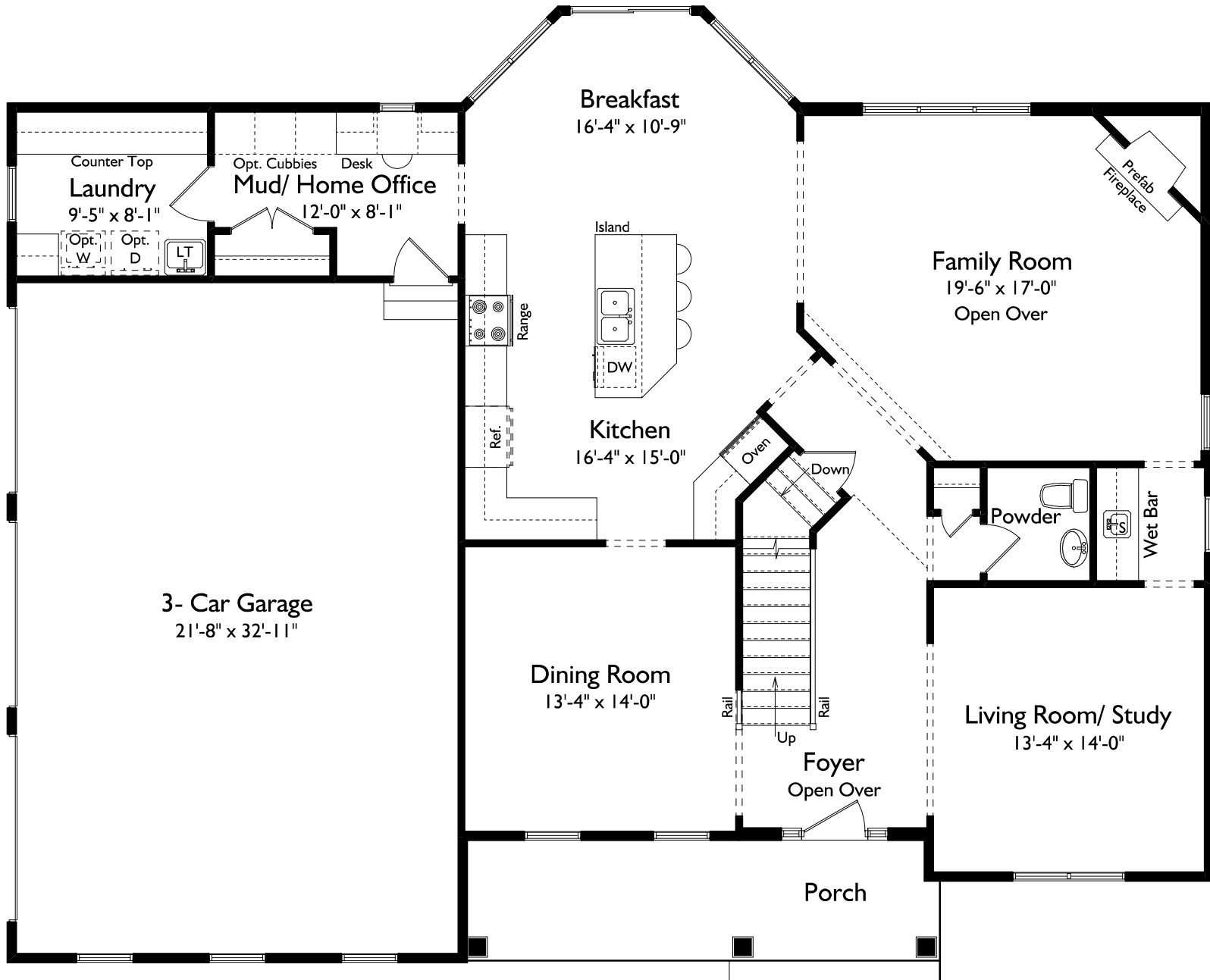
First Floor Plan The Riverchase
