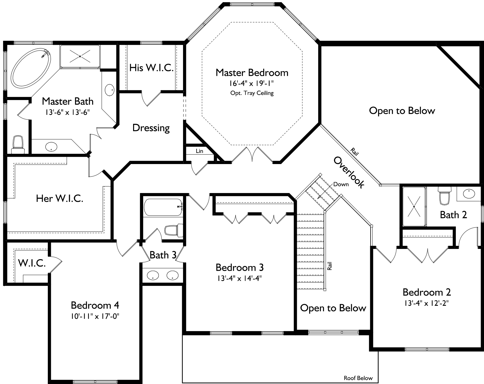
Second Floor Plan The Riverchase
