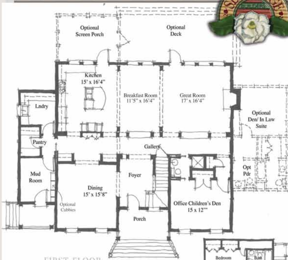
FIRST FLOOR
