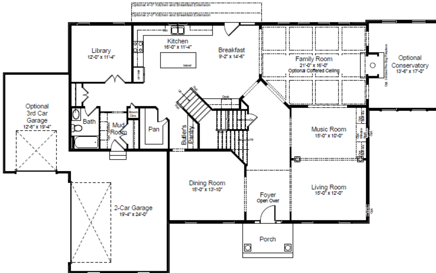
First Floor Plan @ Standard Elevation Hawthorne II 1/28/2011
