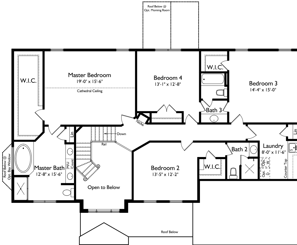
Second Floor Plan The Ashdale
