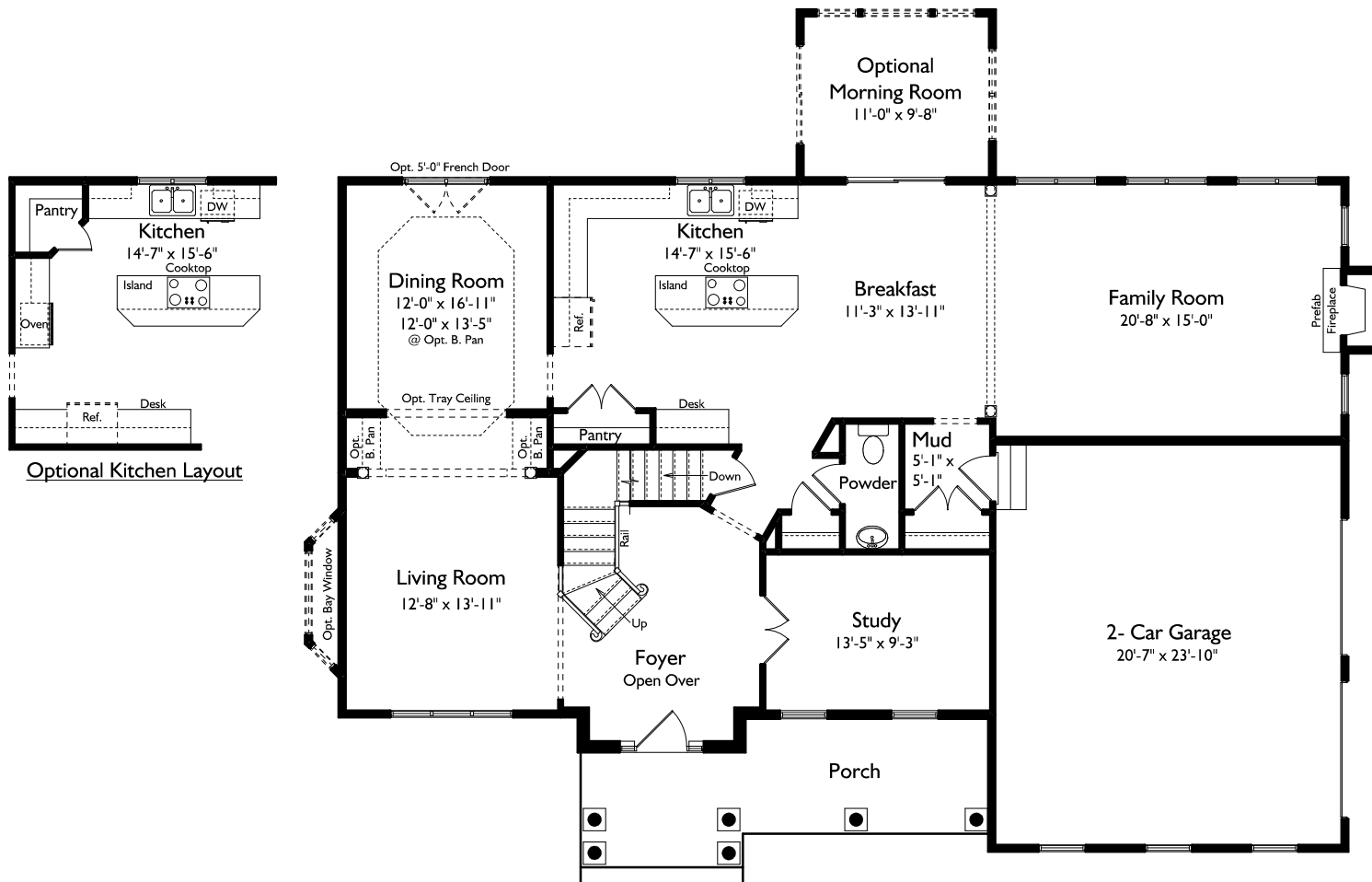
First Floor Plan The Ashdale
